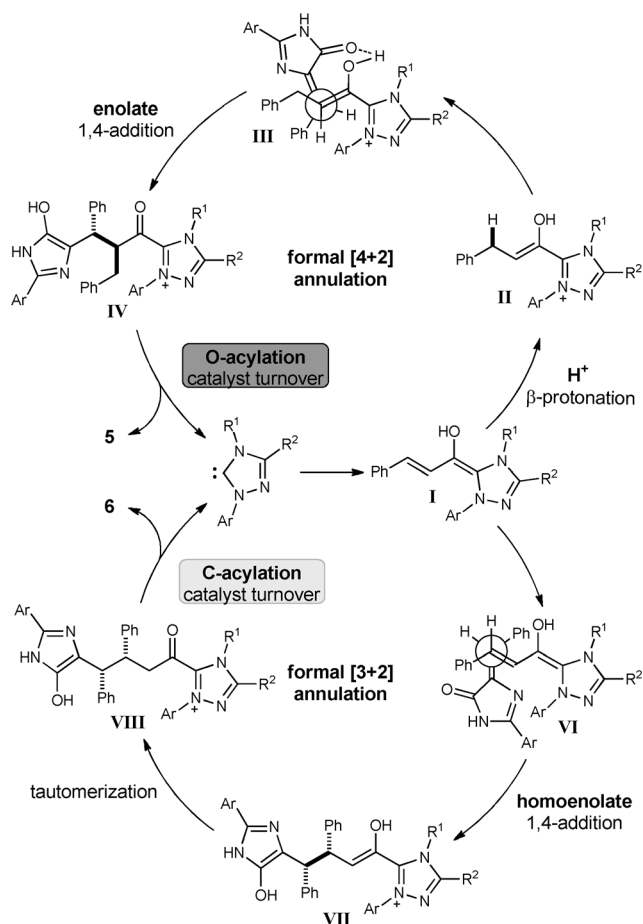
Scheme 3. Proposed reaction pathway.
