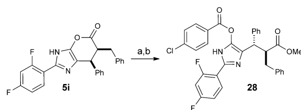
Scheme 4. Representative ring opening. See the Supporting Information for details. Reagents and conditions: a) formic acid (5 % in MeOH), 65 °C, 70 %; b) Et 3 N, 4-chlorobenzoyl chloride, THF, 23 °C, 94 %.
